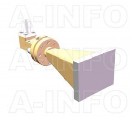
LB-15-20-C-1.85FSPO Standard Gain Horn Antenna 50-65GHz 20dB Gain 1.85mm Female
